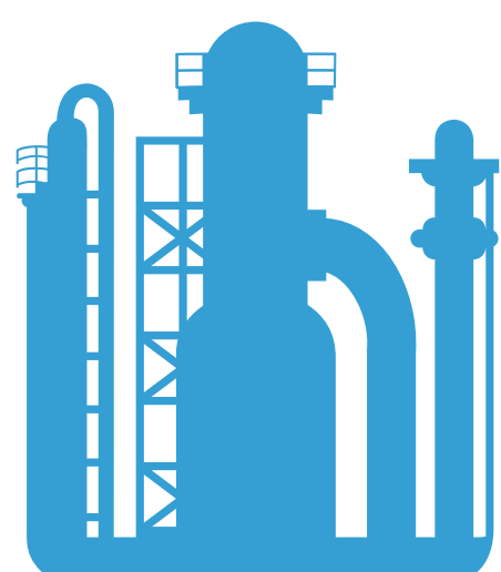
DWSIM
