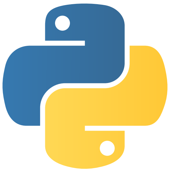
Python
