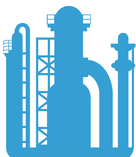
DWSIM
