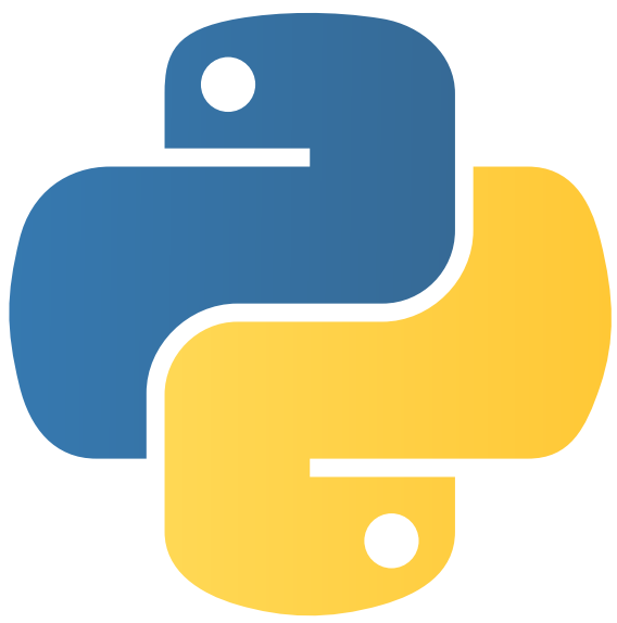
Python
